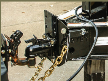
Heavy Duty 4 Bolt Adjustable Coupler
